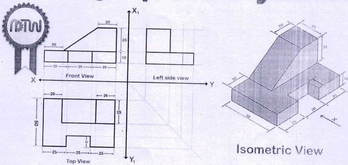
Fig-04 Orthographic from isometric view
