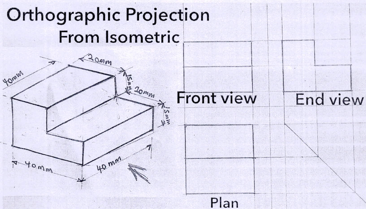
Fig-01 Orthographic from isometric view
